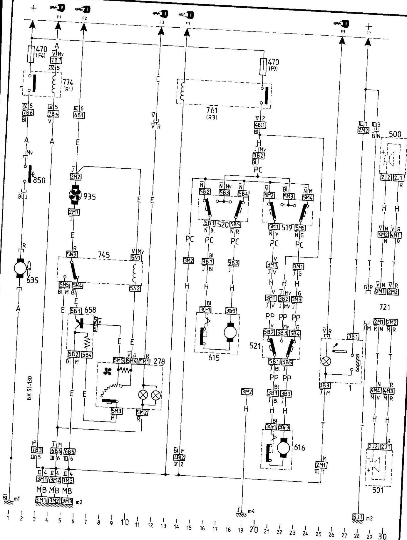
Fig. 13.64 Wiring diagram for BX and BX 14 models October 1988 on - circuit VII
