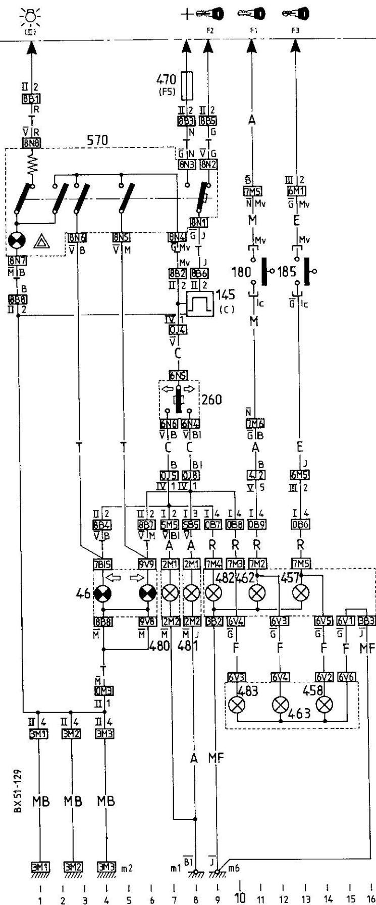
Fig. 13.64 Wiring diagram for BX and BX 14 models October 1988 on - circuit VI
