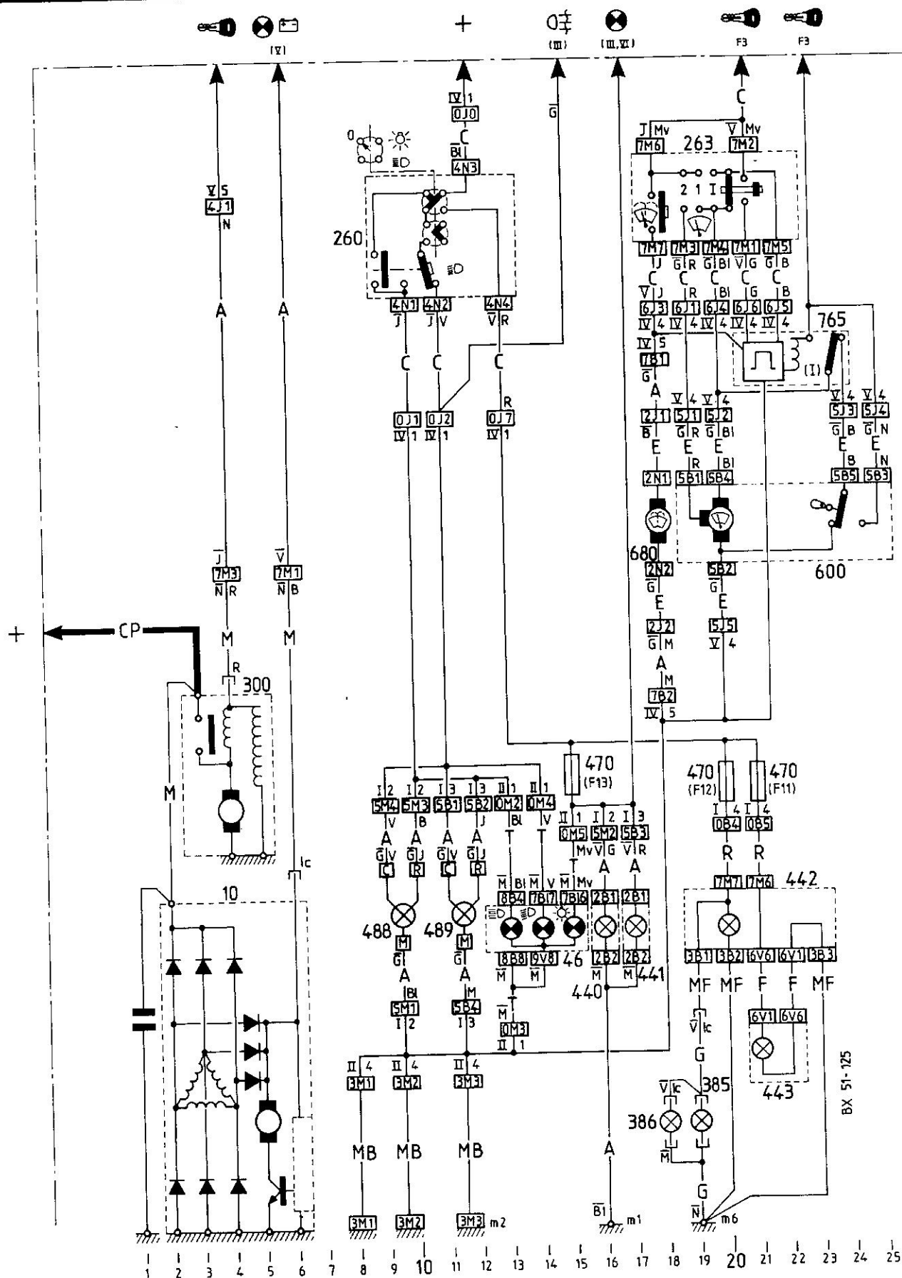
Fig. 13.64 Wiring diagram for BX and BX 14 models October 1988 on - circuit II
